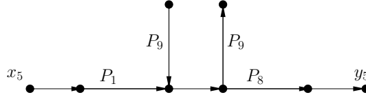
Figure 11: The digraph T_5 .
