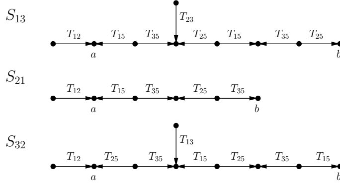
Figure 15: The choosers S_{13} , S_{21} and S_{32} .
