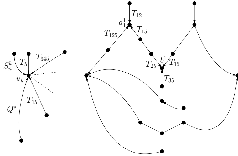
Figure 25: The node u_k and a copy of \tilde{T} .
