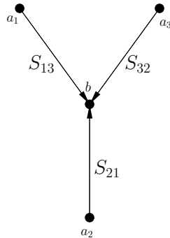
Figure 18: The digraph T' .
