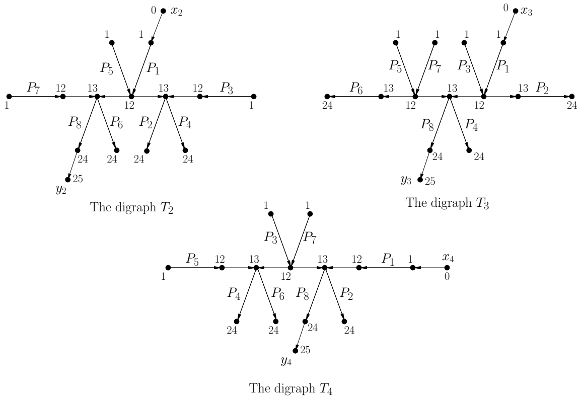
Figure 10: The digraphs T_2 , T_3 and T_4 and some of its levels.
