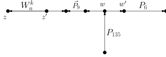
Figure 23: The digraph S .
