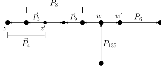
Figure 23: The digraph S .
