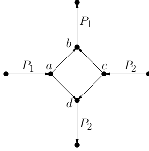
Figure 3: The digraph D .
