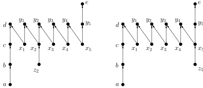
Figure 22: The digraphs W_5^2 and W_5^5 .
